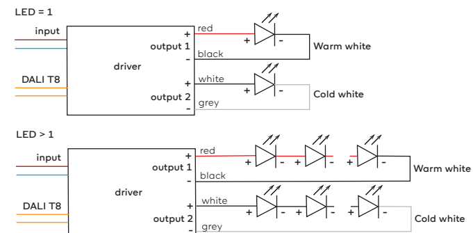
electrical diagram TW
