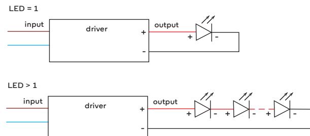
electrical diagram
